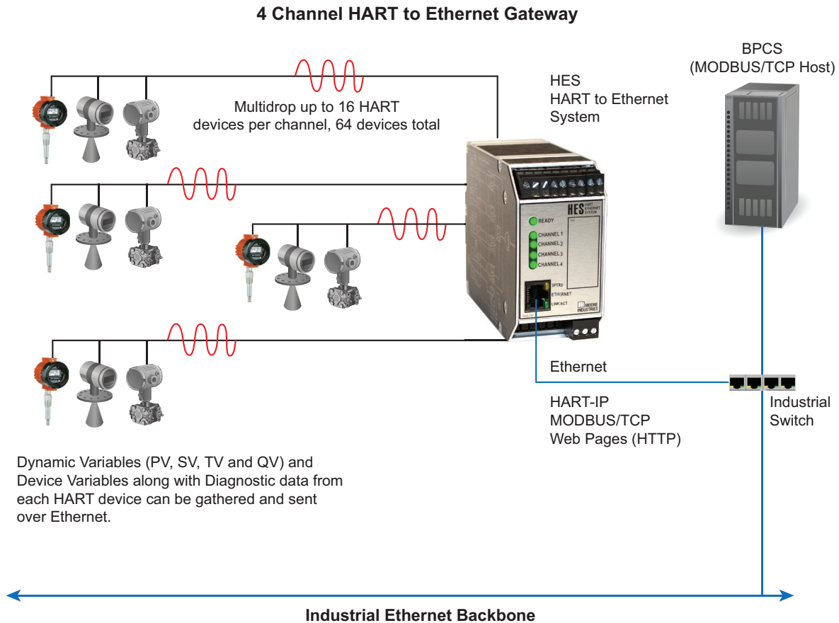
Figure 2. Four Channel HART to Ethernet Gateway can multiplex HART device data from up to 64 devices to deliver HART data to a MODBUS/TCP Host.
