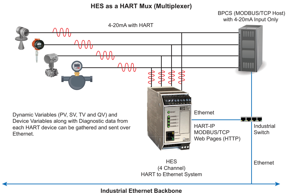
Figure 3 Use the HES to capture up to 128 variables from each of four devices and deliver the data to an asset management system.
